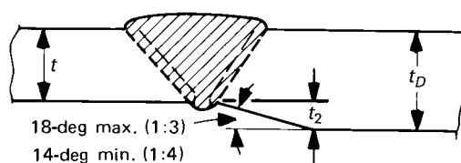
Fig. 13 Bevel for Inside Thickness
