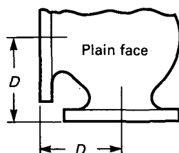
Class 125 Cast Iron
