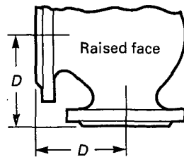
Class 250 Cast Iron and Class 300 Steel
